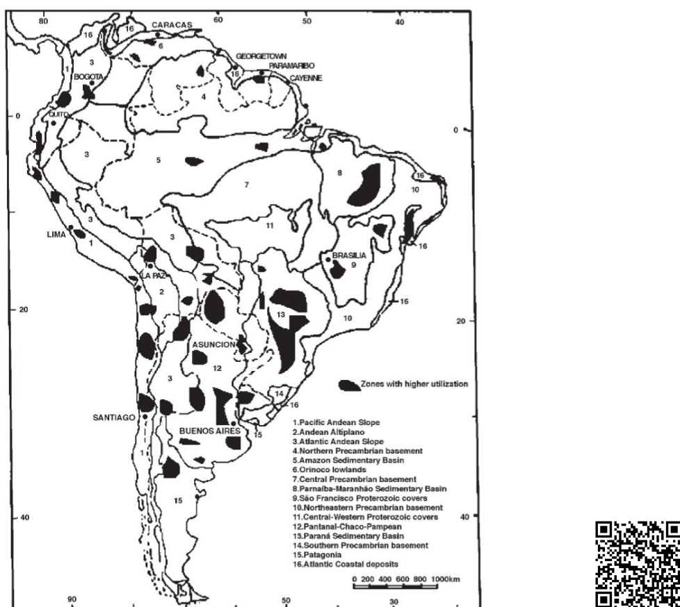
Figure 2-13: South America — Hydrogeological provinces and zones with higher utilization of groundwater. Illustration from Groundwater resources in South America (Rebouças, 1999). For an enlarge version of this image click here or scan the QR code.
