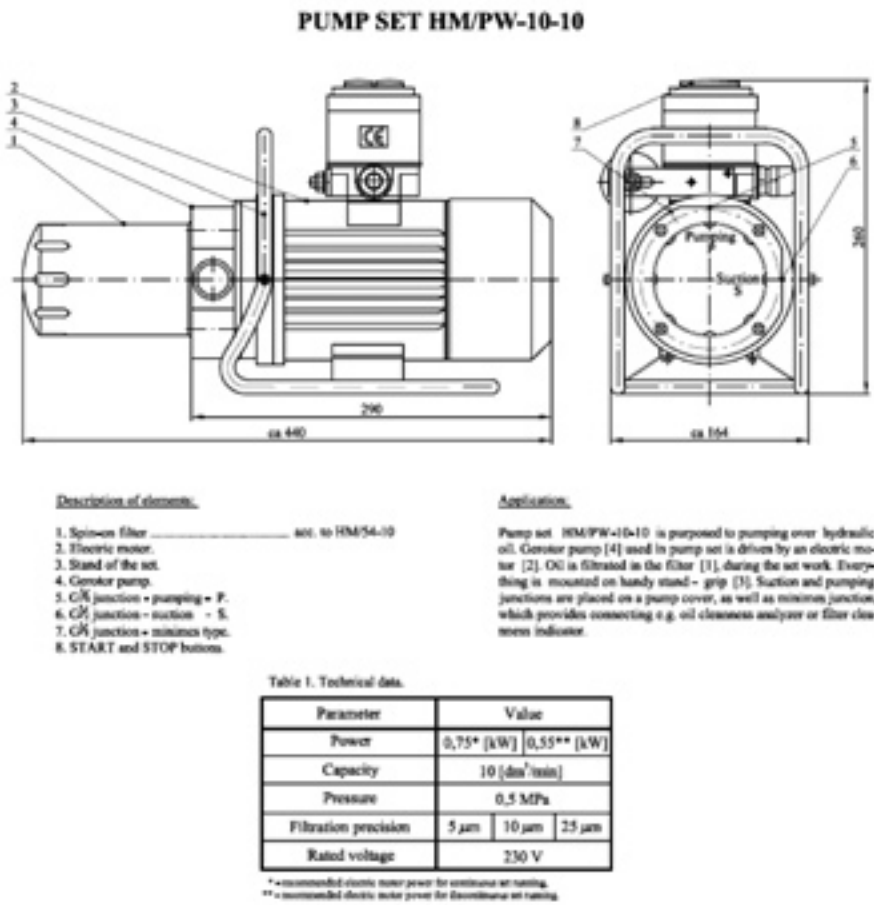
Dwg. 3. Construction of Pump set.
